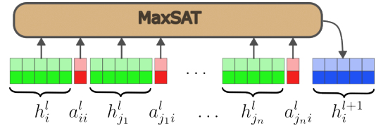
Figure 2. Visualization of the batch version of the MAXSAT (B-MAXSAT-MP), where multiple nodes’ features are considered at once.
